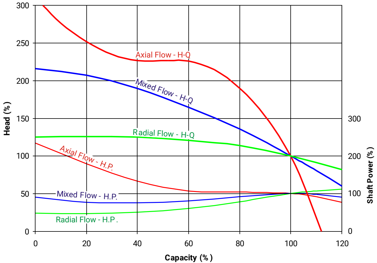
COMPARISON OF H-Q & H.P. CURVES AT 100% OF MAXIMUM EFFICIENCY
