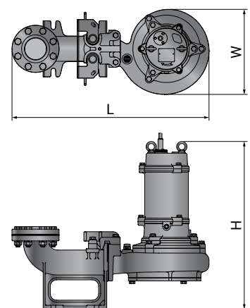
Guide Rail Installation
