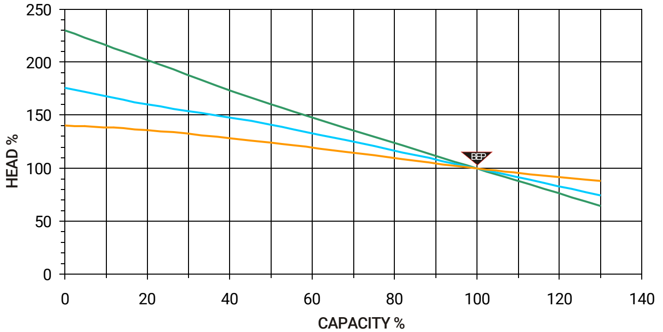
PERCENTAGE RISE FROM BEP TO SHUT OFF HEAD
