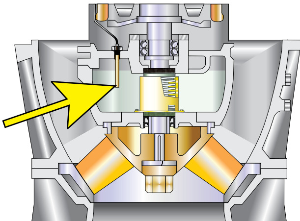
Figure 2 SEAL SENSOR
